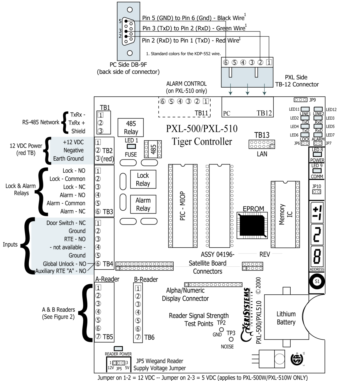
Figure 1: The PXL-500/PXL-510 Controller
