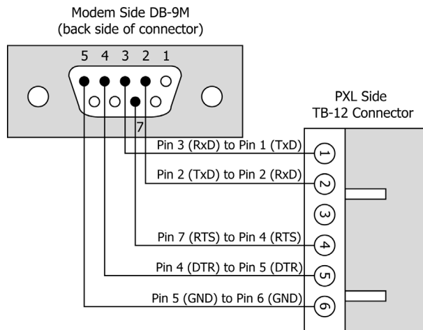
Figure 3: Modem/DB-9M to PXL/TB-12 Serial Port Connection
