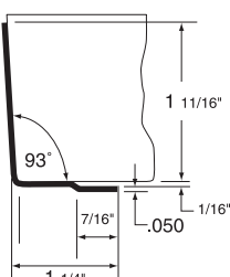
No. EG13 (single side)
