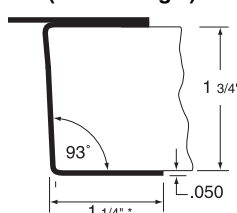
No. EG08A (with Astragal)
