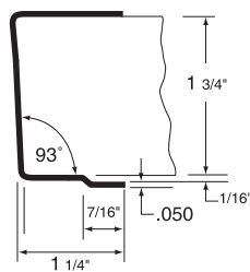
No. EG15 (single side)
