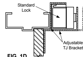
FIG. 1D Top Jamb Installation
