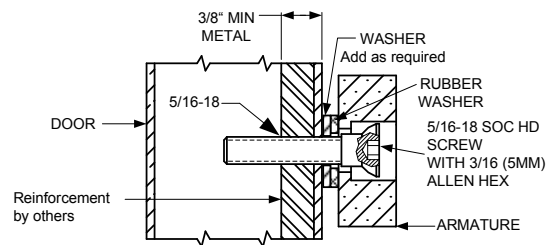
FIG. 2C REINFORCED DOOR
