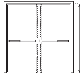
Door Opening Height is measured from finished floor to frame rabbet on door side.
