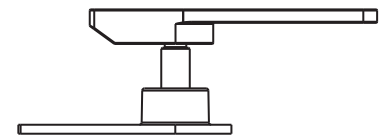
Adjustable End Load Bottom Pivot (PV-ENDLOAD)
