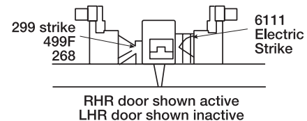
4854/9854 – Using one electric strike
