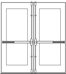
Two surface mounted vertical rod devices—same direction*
