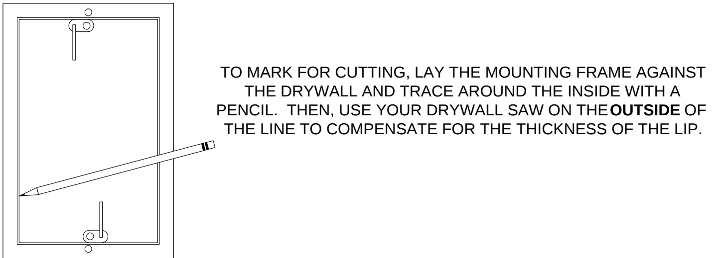
FIG. 1: INSTALLING THE DRYWALL MOUNTING FRAME
