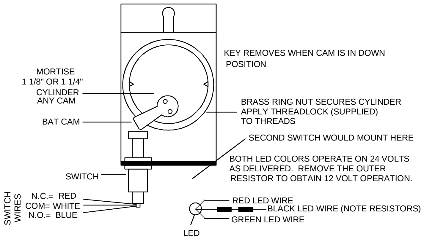
FIG 2: MK PHYSICAL AND ELECTRICAL DETAILS
