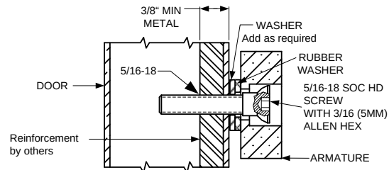
FIG. 2C REINFORCED DOOR
