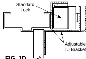
FIG. 1D Top Jamb Installation
