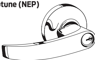
Neptune (NEP)
