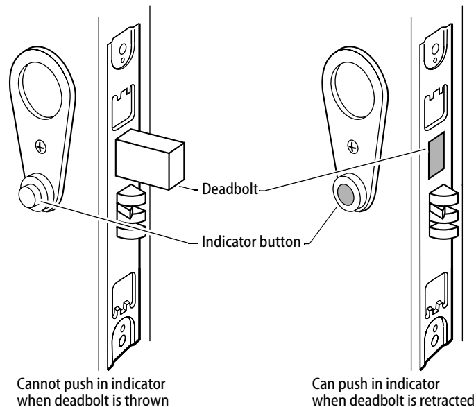
Figure 3 — Testing the hotel indicator for proper operation
