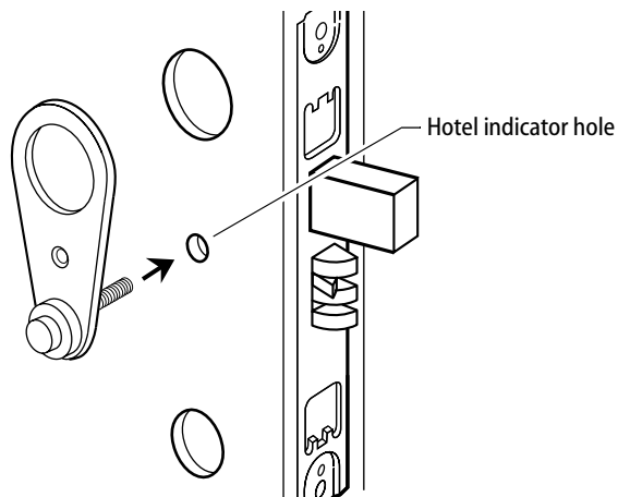
Figure 2 — Placing the hotel trim plate against the door
