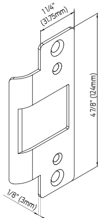
NC450-LBM 1 1/4" x 1/8" x 4 7/8" (31.75mm x 3mm x 124mm)
