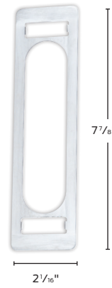
#33A-WDA Cover plate kit for 360 Series controls
