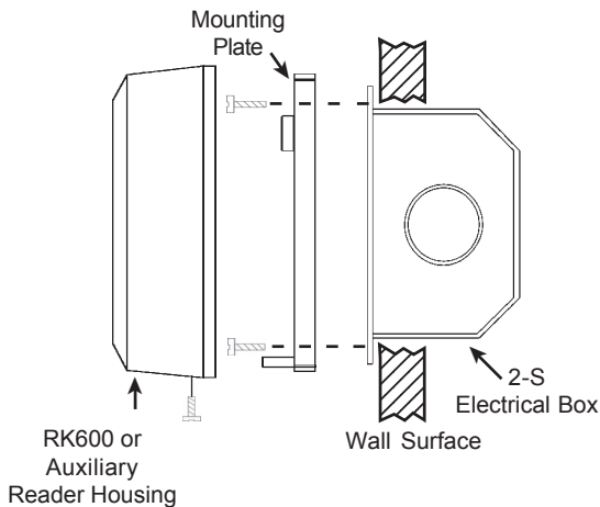
Figure 4 - Basic Installation
