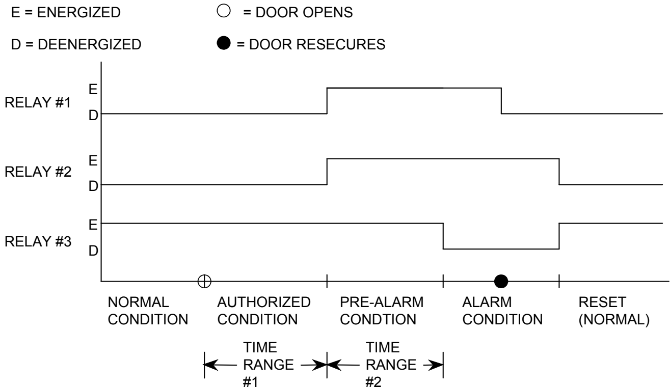
FIG. 2: BASIC OPERATION OF THE DPA
