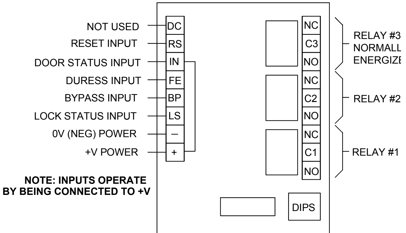
FIG. 1: CIRCUIT BOARD OVERVIEW
