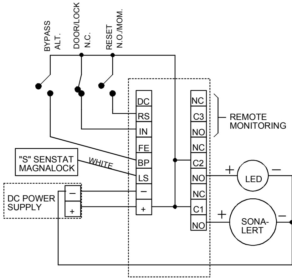
FIG. 2: COMPLETE WIRING EXAMPLE
