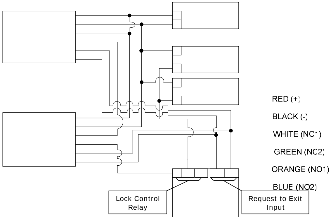
Figure 14 – Double Door with Access Control
