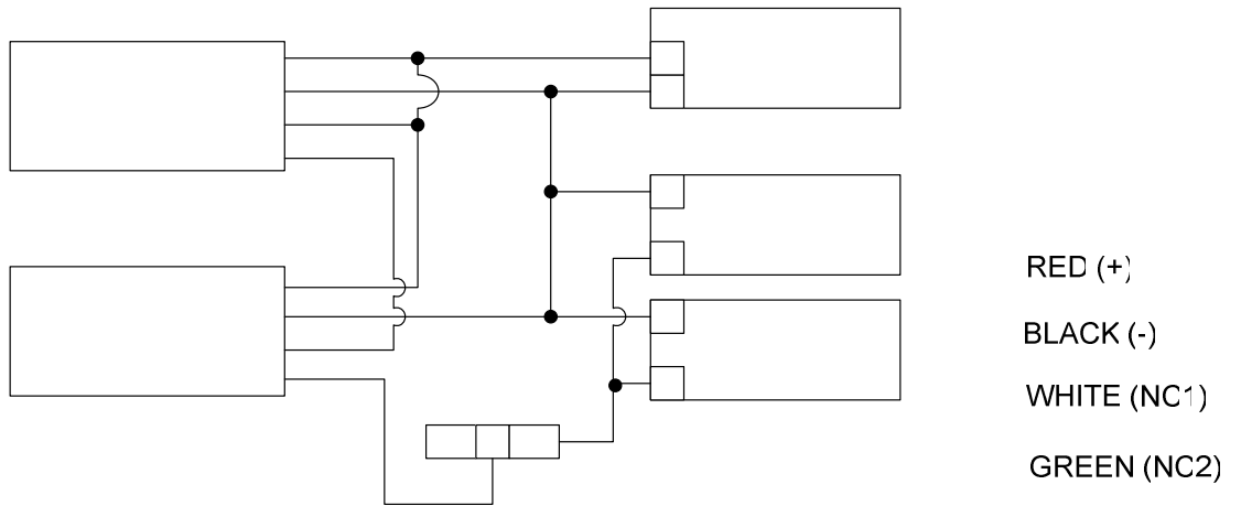
Figure 12 – Double Door (No Access Control Unit)
