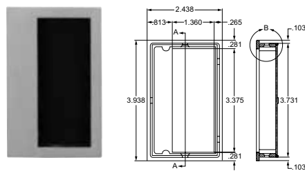
962 Rectangle flush pull with black inset
