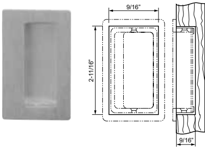
960 Rectangle flush pull
