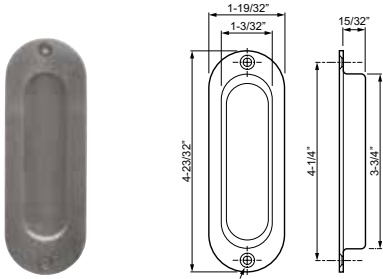
919 Oval flush pull
