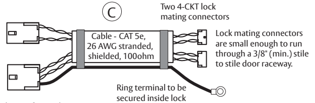
PoE Door Harness Assembly
