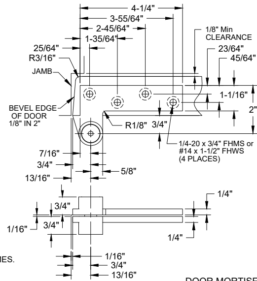
DOOR MORTISE "A"
