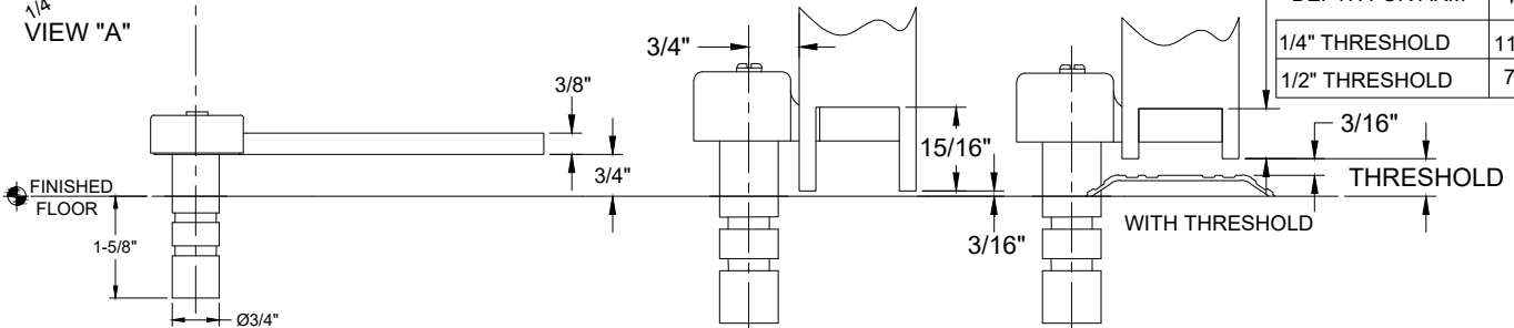
DOOR MORTISE "A"
