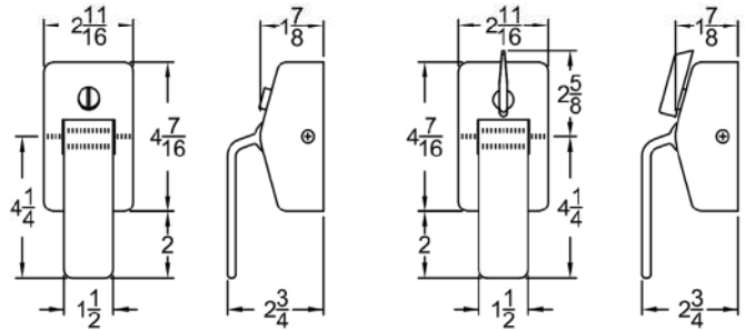
Override Knob
